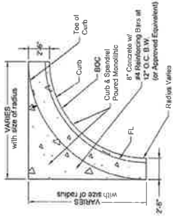
8" SPANDREL, CURB AND GUTTER
