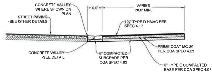
3 PAVING SECTION AT HAMMER HEAD
