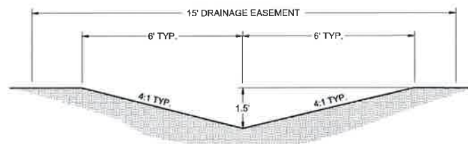
2 TYPICAL CHANNEL SECTION
