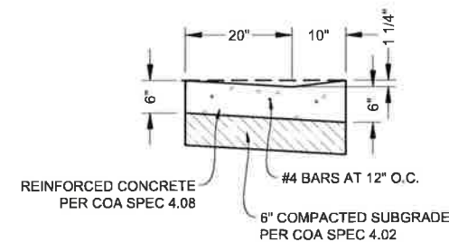
5 TYPICAL LAY-DOWN CURB
